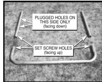
6 Lay one U-shaped leg piece, one leg extension, and one plugged leg extension on the ground. (Plugged holes are for optional Safety Enclosure.)
