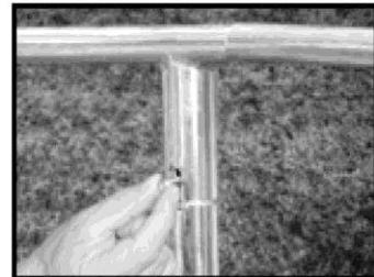
9 Secure U-leg to top-rail with large set-screws on each side.
