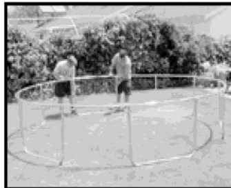
11 Continue until all U-legs are in place.
