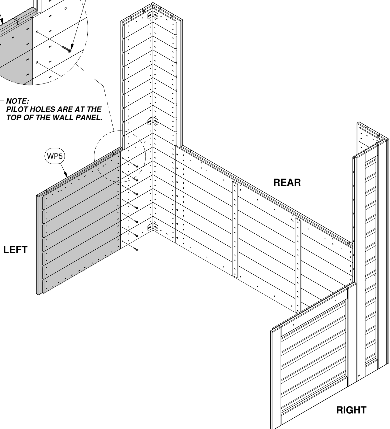
537 (x7) SCREW - 1"
