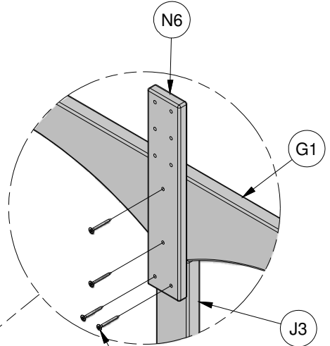
538 (x4) SCREW - 1 1/2"
