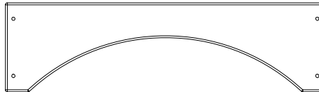
K3 | TRIM - W4L11680 (x1) | 5/8"x5 1/4"x18 15/16" (16x134x481)
