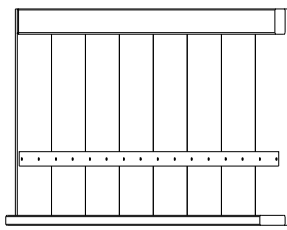
RP8 | ROOF PANEL - W2A02640 (x1) | 1 3/8"x20 1/4"x26 5/8" (71x515x675)
