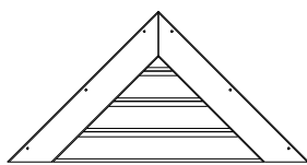
GP2 | GABLE PANEL - W2A02635 (x1) 1 1/16"x17 7/8"x35 13/16" (27x402x803)
