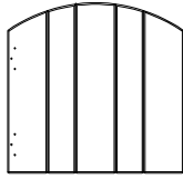
GP1 | GATE PANEL - W2A02554 (x1) | 1 1/16"x14 5/16"x14 7/8" (27x364x378)
