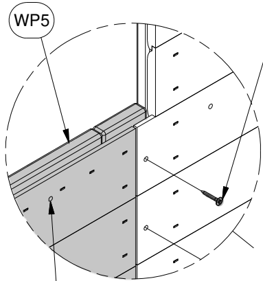
537 (x7) SCREW - 1"
