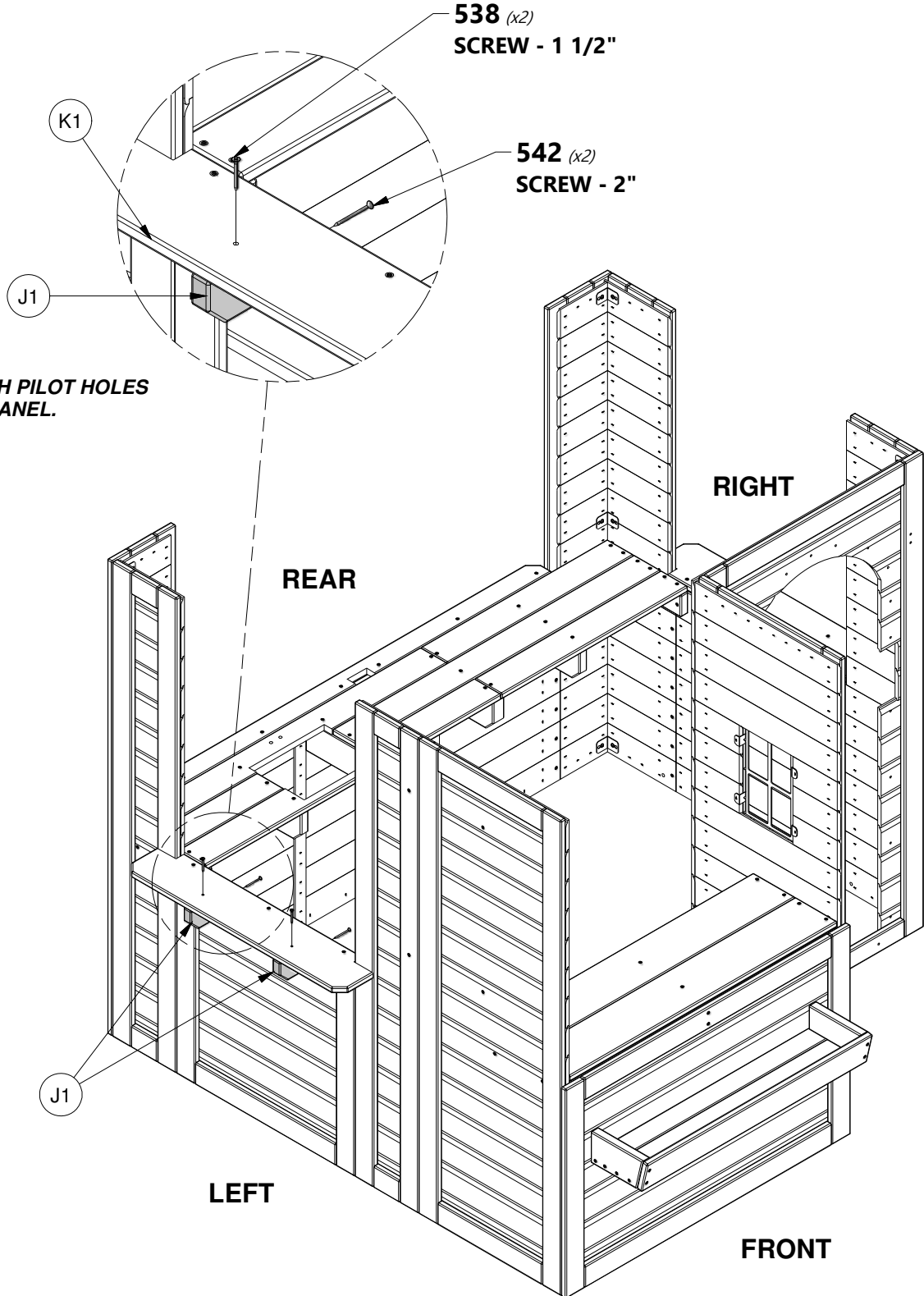
H100538 | SCREW PFH SD (x2) | 8x1 1/2
