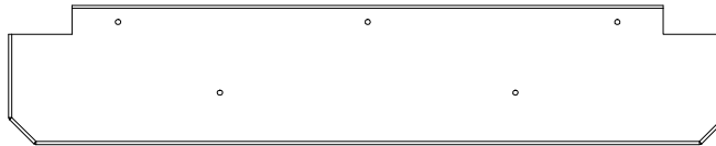
K1 | WINDOW TRIM - W4L08948 (x2) | 5/8"x5 1/4"x27 3/16" (16x134x690)
